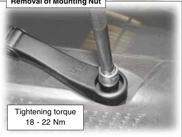
Removal of Mounting Nut
