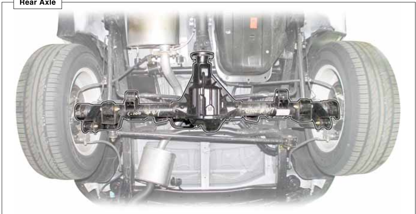
Rear Axle
