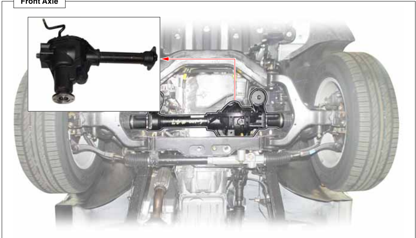
Front Axle
